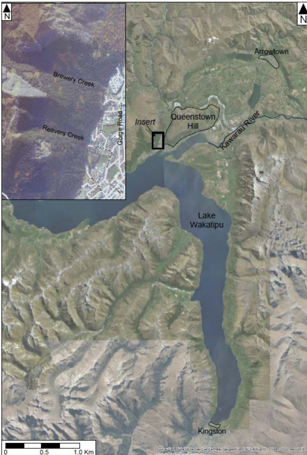
Figure C 1: Annotated aerial photograph outlining the distribution of townships and geomorphic features of relevance to the geomorphic history of the wider Queenstown region.
