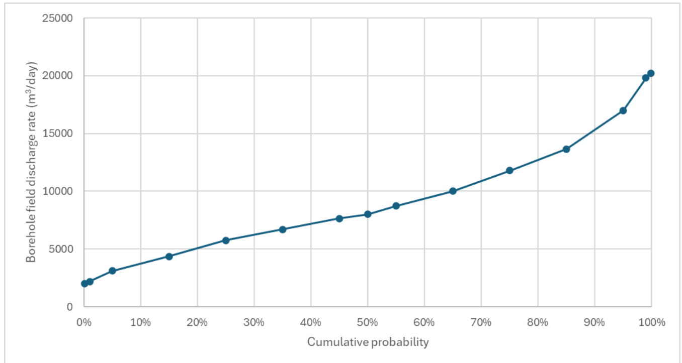
Figure E-3 Combined borehole discharge rate (total of 10 bores)
