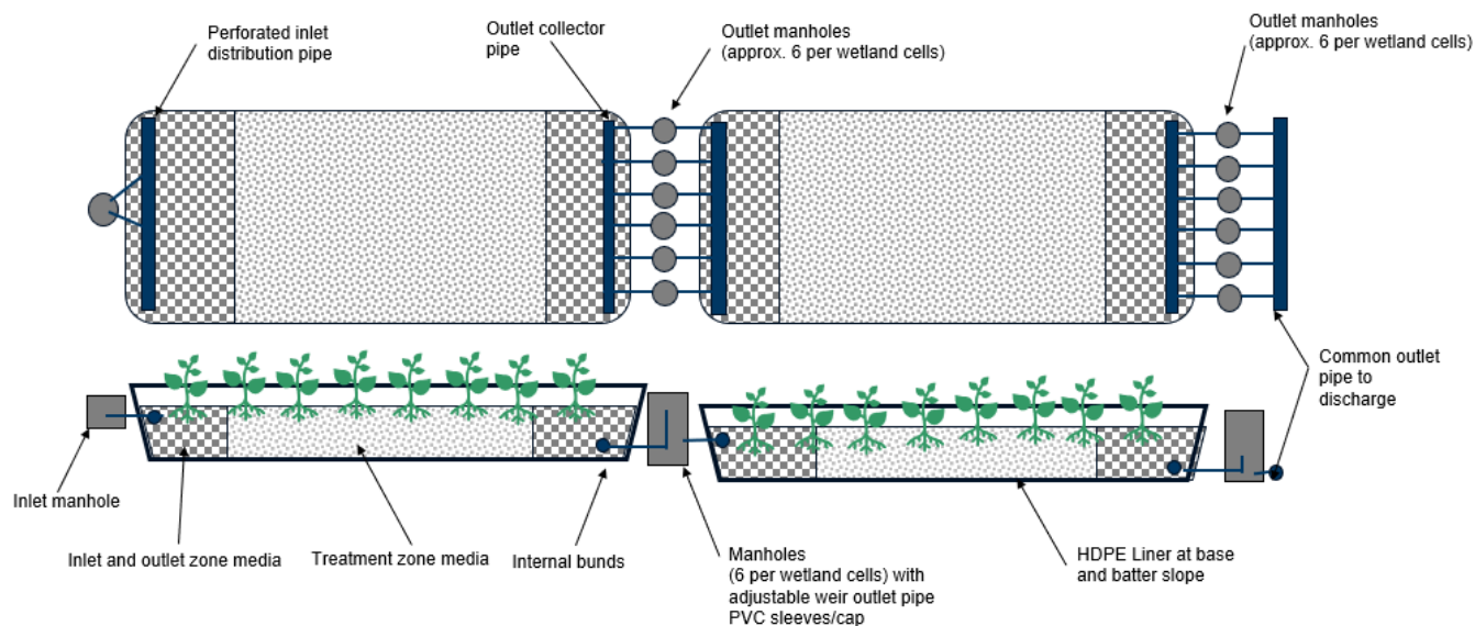
Figure 17 Subsurface wetland conceptual schematic
