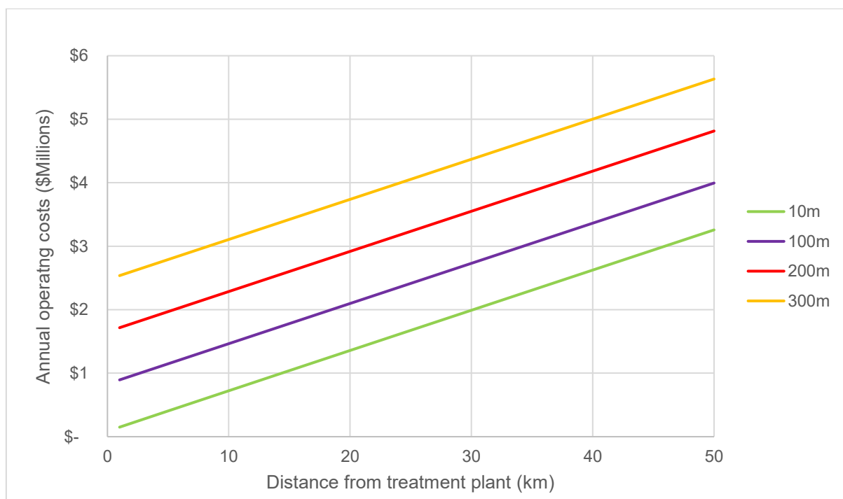
Figure 4 Annual operating costs for a range of distances and elevations
