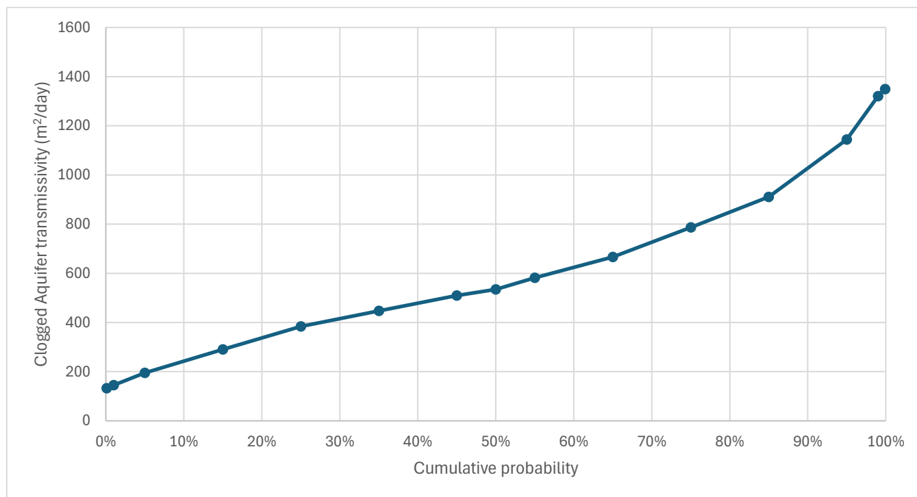
Figure E-1 Range of transmissivity and clogging for the boreholes on Frankton.
