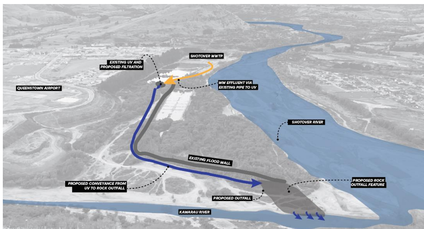
Figure 25 Option A Rock outfall schematic illustration
