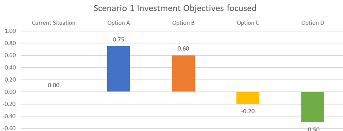
Figure 33 Weighted short list scores - Scenario 1: Investment Objectives Focused
