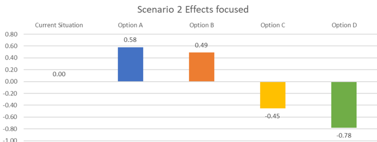
Figure 34 Weighted short list scores – Scenario 2: Effects focused
