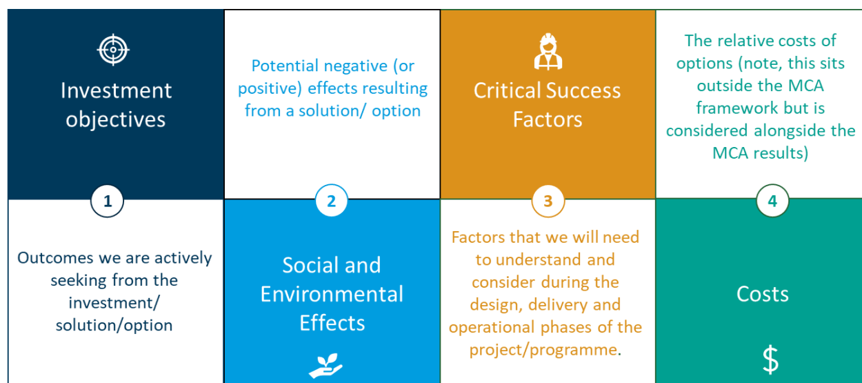
Figure 2 MCA framework
