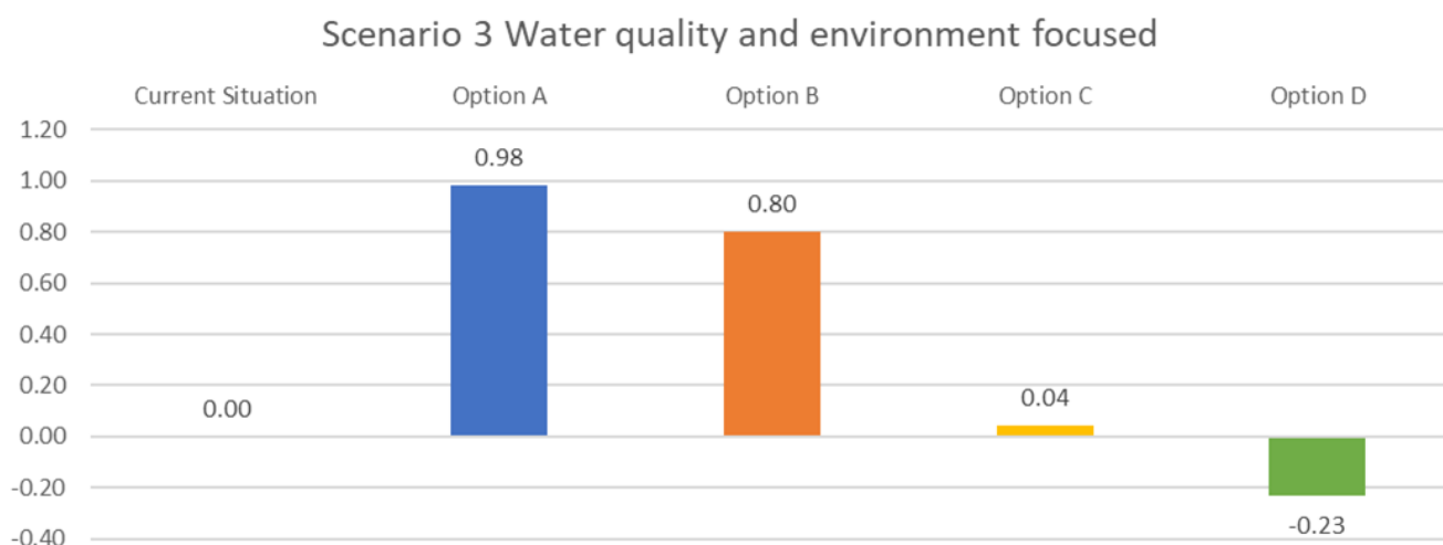
Figure 35 Weighted short list scores – Scenario 3: Water quality and environment focused
