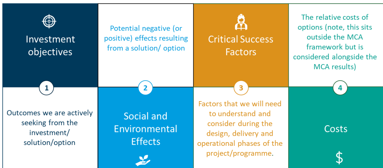
Figure 32 MCA framework
