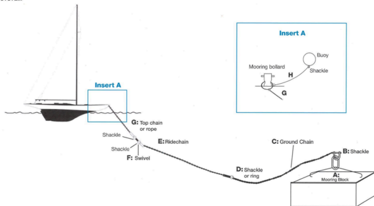
FIGURE 1 MOORING SYSTEM
